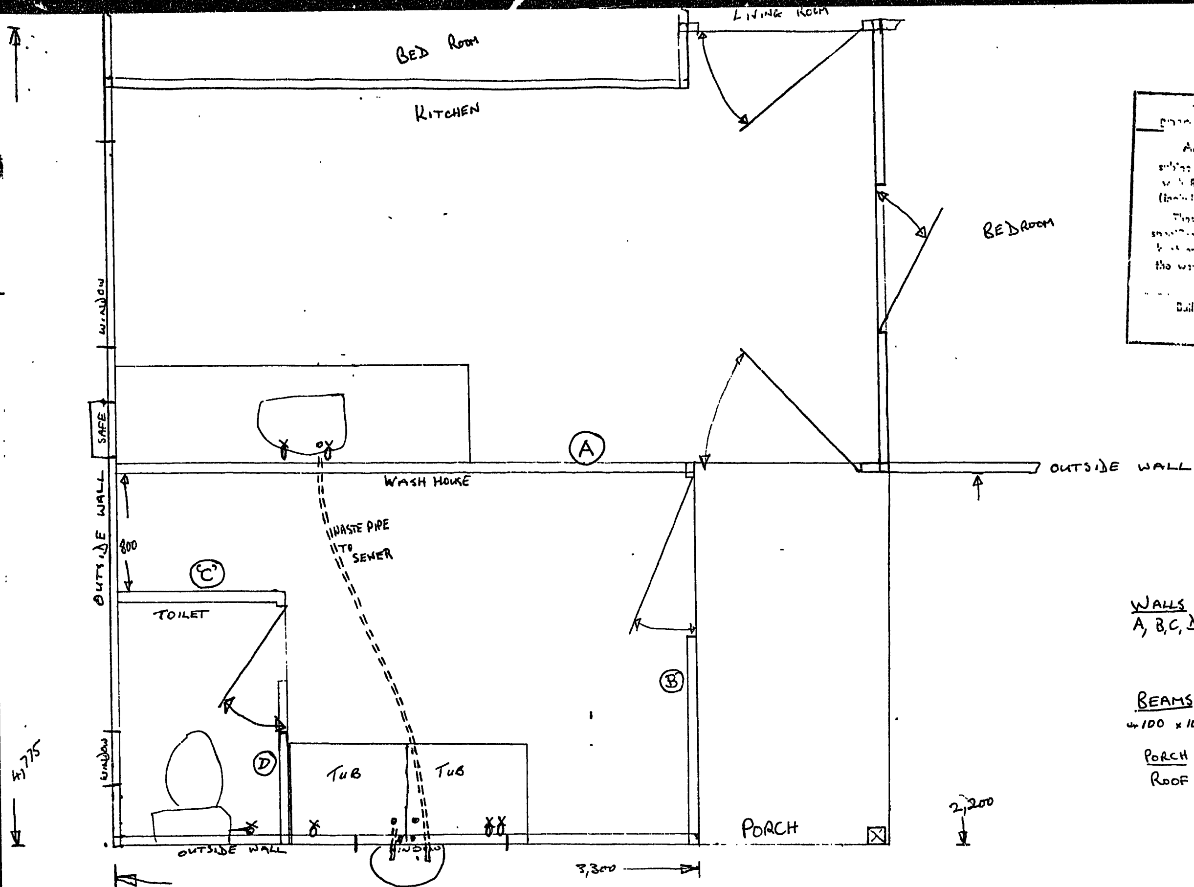
FLOOR PLAN BEFORE ALTERATIONS 50 mm = 1 m. 15 EAST AVENUE
