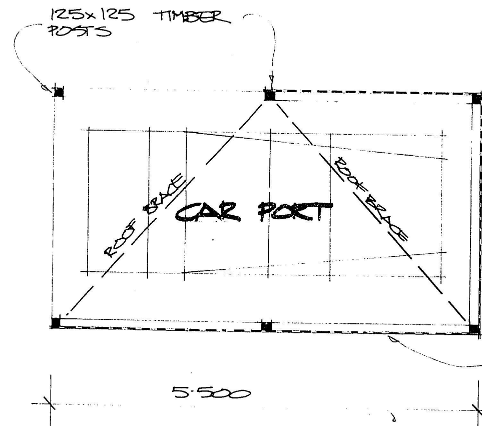
FLOOR PLAN 1:50
